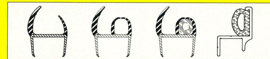
Sea-Lok Standard
