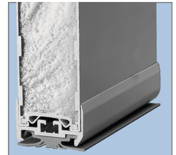
Heavy duty aluminum channel and flexible seal features a rigid landing surface to protect seal.
